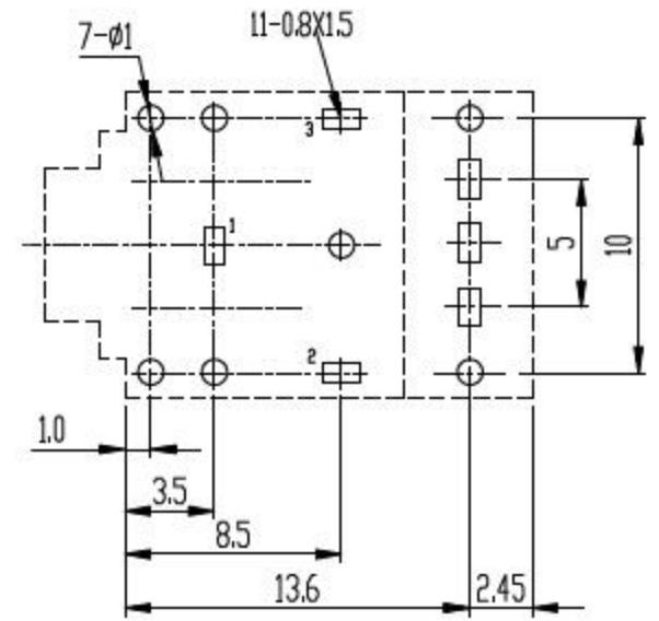
PCB LAYOUT TOP-SIDE VIEW
