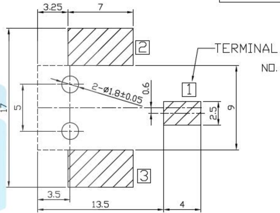
RECOMMENDED P.C.B. LAYOUT UNSPECIFIED TOLERANCE: ±0.05 (COPPER-TOP VIEW)
