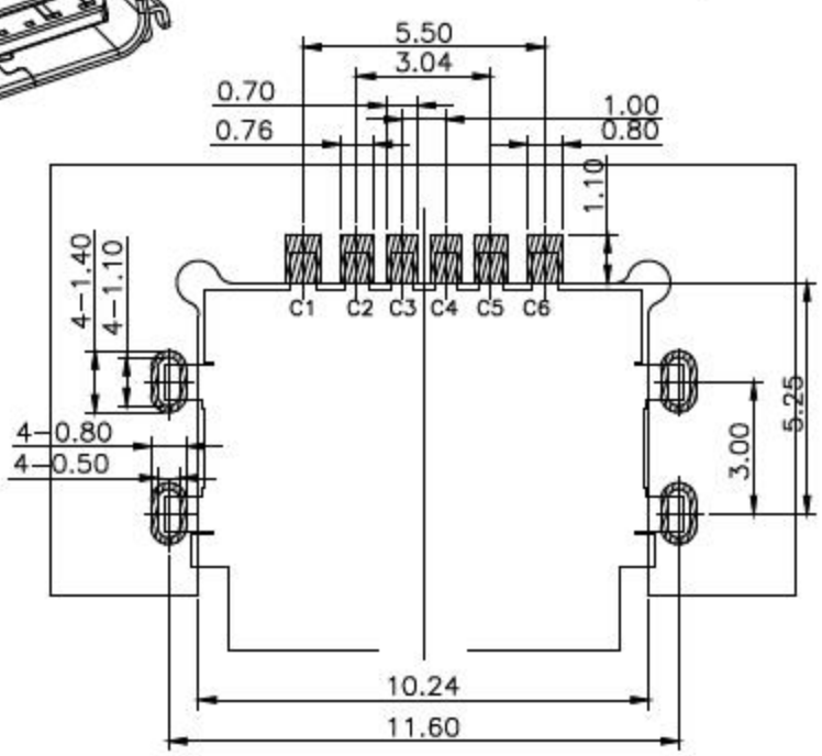
RECOMMENDED P.C.B. LAYOUT TOLERANCE UNSPECIFIED ±0.05mm
