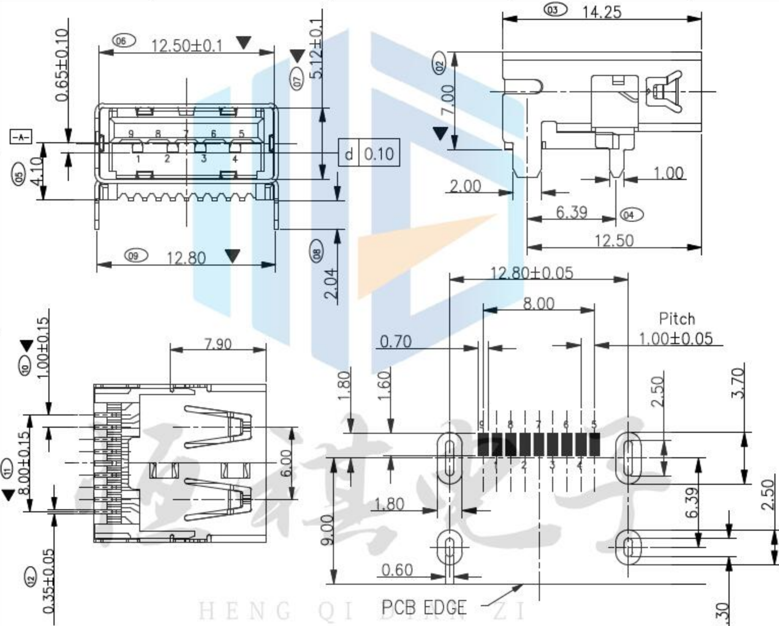
RECOMMENDED PCB LAYOUT TOLERANCE: ±0.05mm
