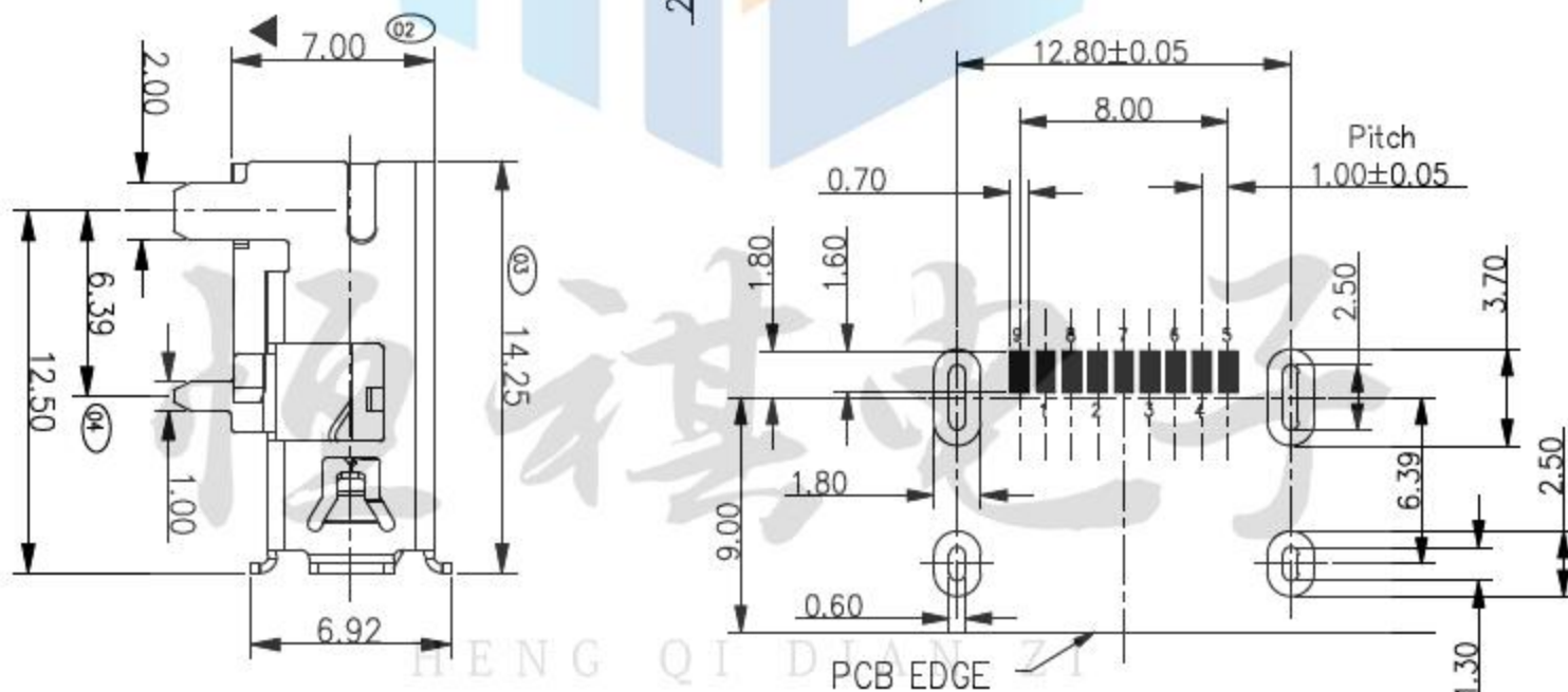
RECOMMENDED PCB LAYOUT TOLERANCE: ±0.05mm
